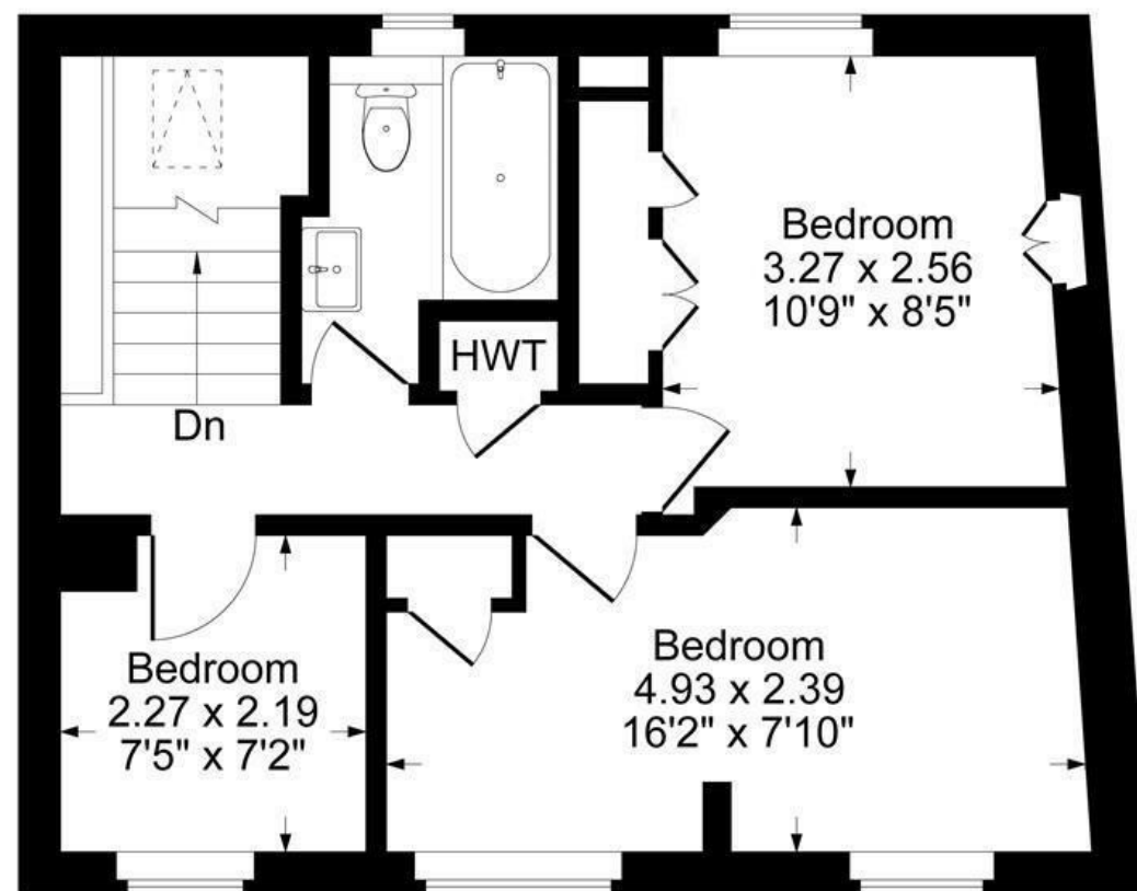
First Floor
